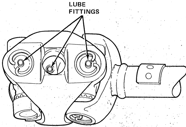
Fig. 2E-6 Double Cardan Joint Lube Fittings
